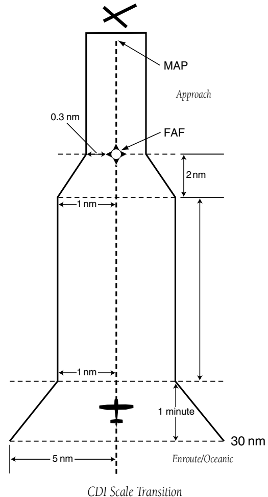
Figure D-7 CDI Scale Transition
