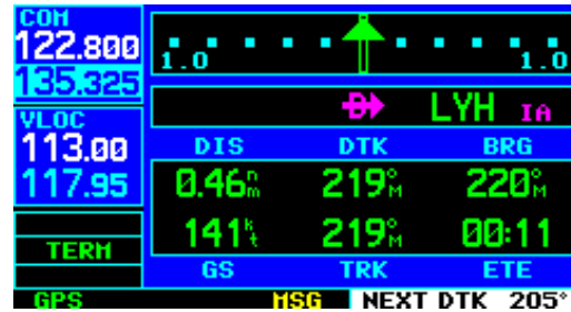
Figure D-6 CDI at 1 nm Scale
